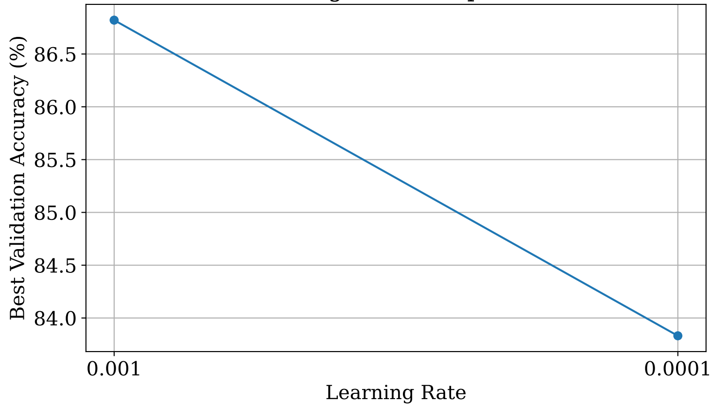
Learning Rate Comparison
